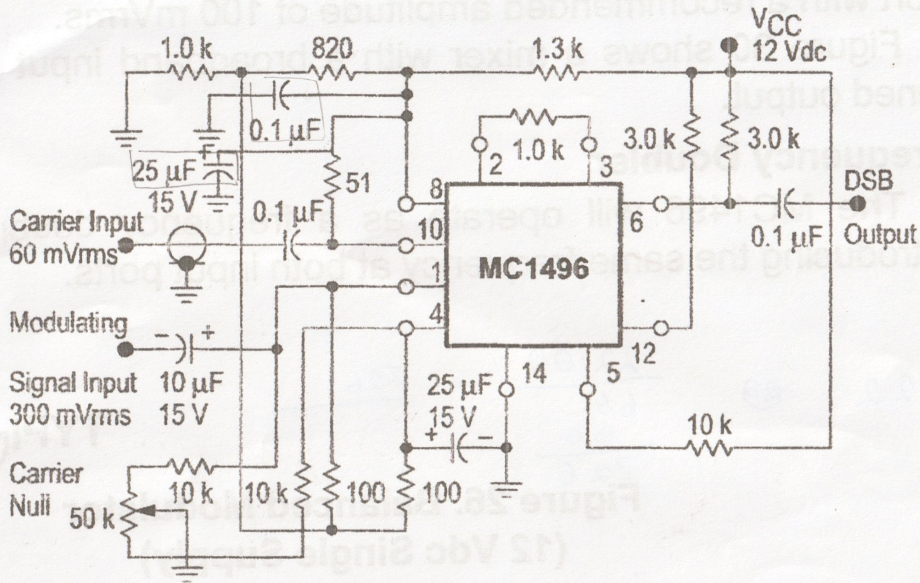
Figure 26. Balanced Modulator (12 Vdc Single Supply)
